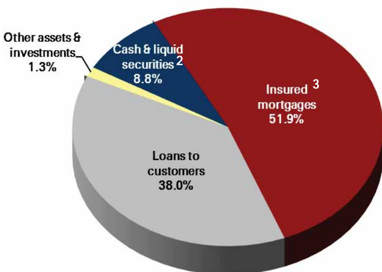
Asset profile
