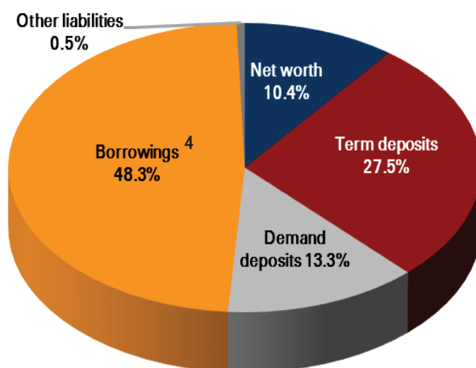
Liability profile
